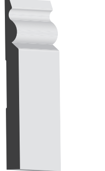
No. 1867 15mm X 7-1/4" X 16" Part No. 10001026 MDF Prm
