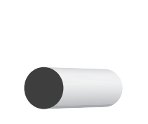
No. 233 1-1/4" X 1-1/4" X RL Part No. 10000739 Pine 1-1/4" X 1-1/4" X 16" Part No. 10033372 LVL 1-5/16" X 1-5/16" X 8" Part No. 10003265 Vinyl 1-5/16" X 1-5/16" X 6" Part No. 10003266 Vinyl
