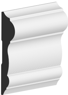
NO. 297 5/8" X 3" X 16' Part No. 10000515 Primed Fingerjoint Pine
