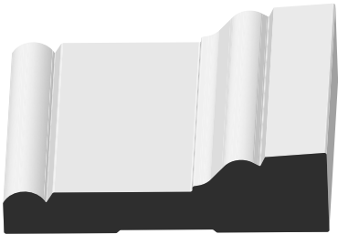
NO. ADAMS 1-1/16" X 3-1/2" X 16' Part No. 10004132 Primed Fingerjoint Pine 1-1/16" X 3-1/2" X 88" Part No. 10126162 Primed Fingerjoint Pine
