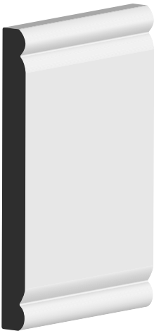
NO. 959H 7/16" X 4-1/2" X 16' Part No. 10001242 Primed Fingerjoint Pine
