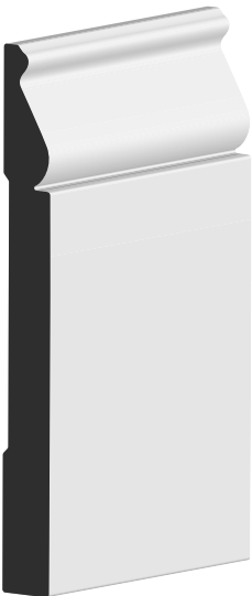
NO. 5163 9/16" X 5-1/4" X 16' Part No. 10000627 Primed Fingerjoint Pine
